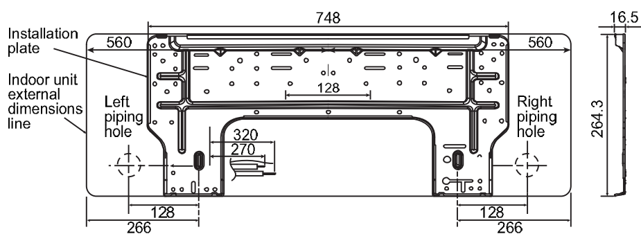
Relative position between the indoor unit and the installation plate &lt;Front View&gt;
