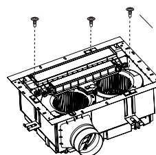
Self-tapping screws \phi 4 \times 13 自攻螺絲 \phi 4 \times 13
