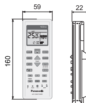
<Remote Control>
